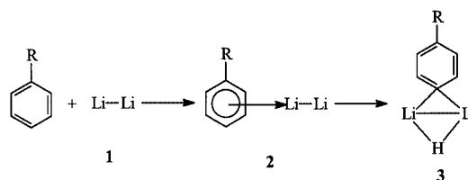
Scheme 5. Key mechanistic steps in aromatic C–H bond activation using lithium atoms
