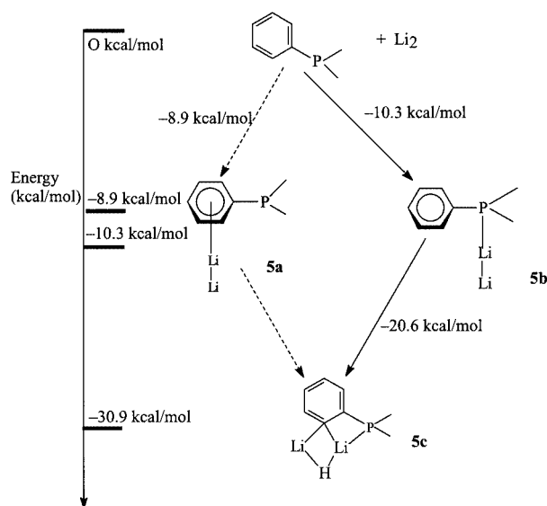
Figure 6. Calculated reaction mechanism for the co-condensation of lithium atoms with dimethylphenylphosphane
