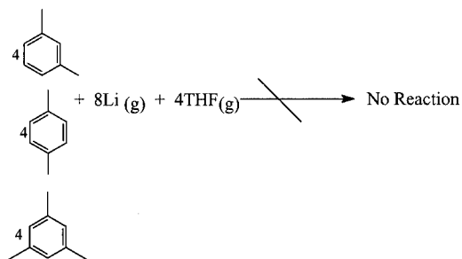
Scheme 1. Failed reaction of lithium atoms with +I-substituted benzene derivatives
