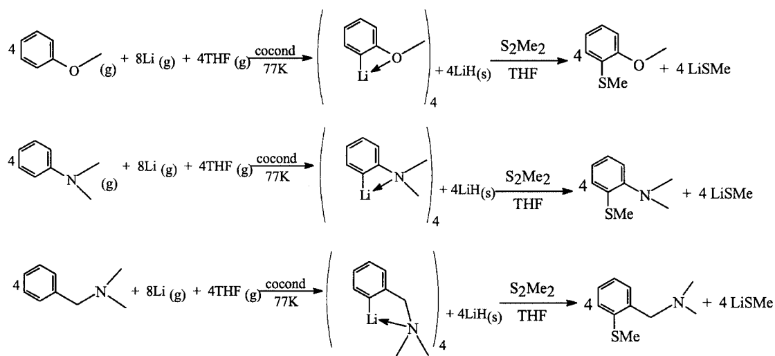
Scheme 3. Reaction of donor-substituted aromatic compounds with lithium atoms in THF
