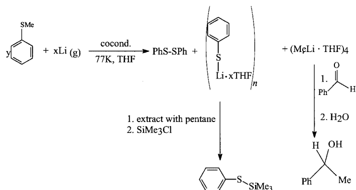
Scheme 4. Co-condensation of lithium atoms with thioanisole in the presence of THF
