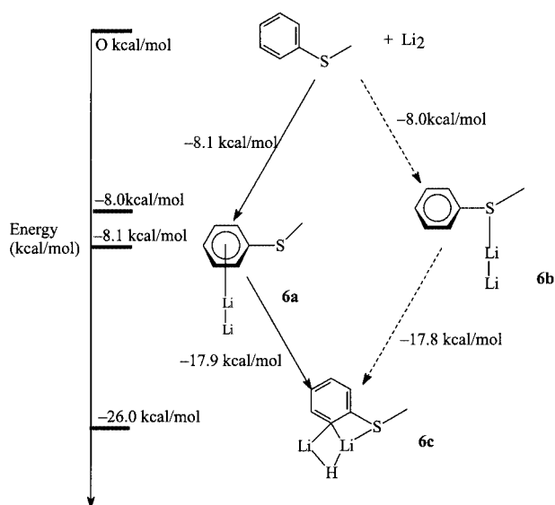
Figure 7. Calculated reaction mechanism for the co-condensation of lithium atoms with thioanisole
