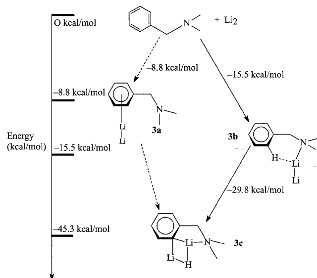
Figure 4. Calculated reaction mechanism for the co-condensation of lithium atoms with benzylamine
