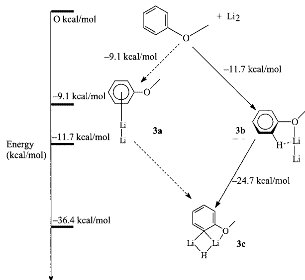
Figure 3. Calculated reaction mechanism for the co-condensation of lithium atoms with anisole
