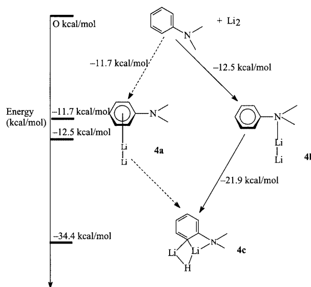
Figure 5. Calculated reaction mechanism for the co-condensation of lithium atoms with N,N -dimethylaniline
