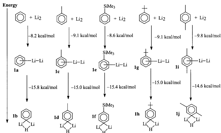
Figure 2. Calculated reaction enthalpies for +I-substituted benzene derivatives and \text{Li}_2
