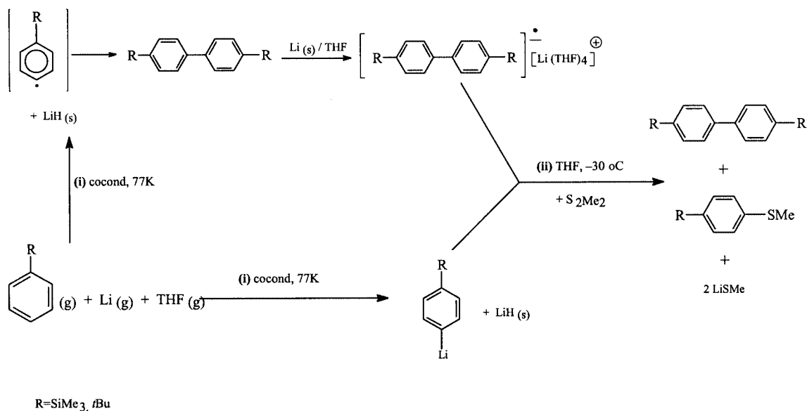
Scheme 2. The reductive coupling of +I-substituted benzene derivatives by lithium atoms
