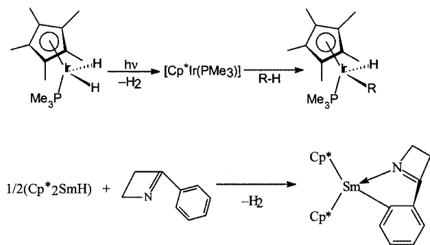
Figure 1. Selected examples of C–H bond activation using metal complexes
